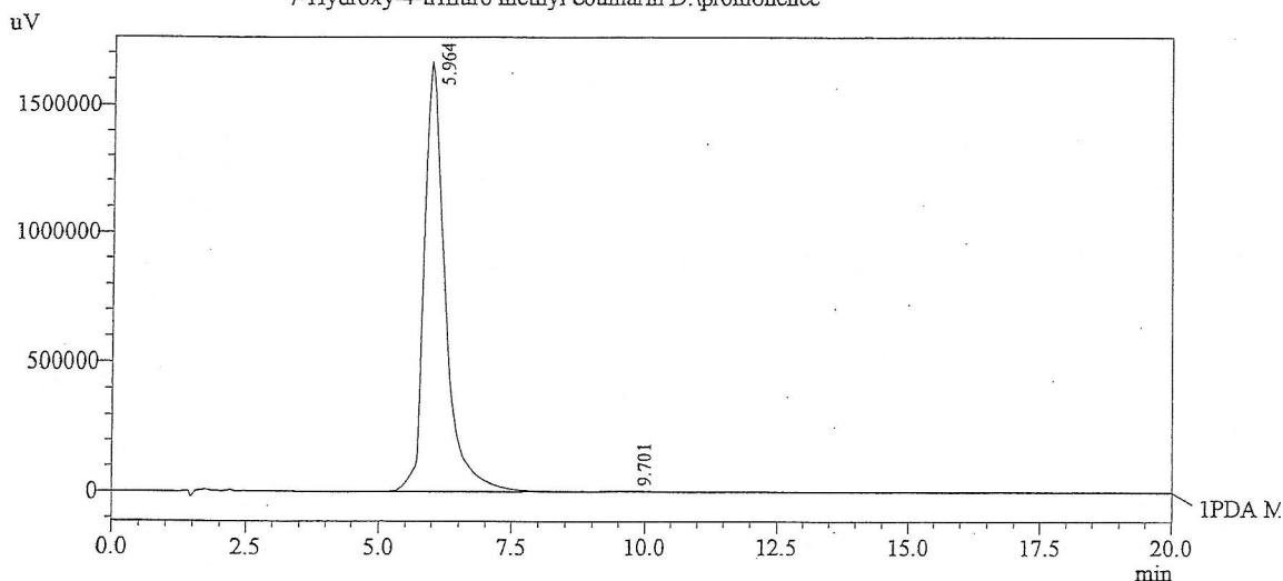
Chromatogram 7-Hydroxy-4-trifluoro methyl coumarin D:\promonence
